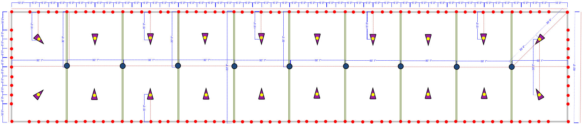
60' x 300' Pole Tent - Pole Placements
